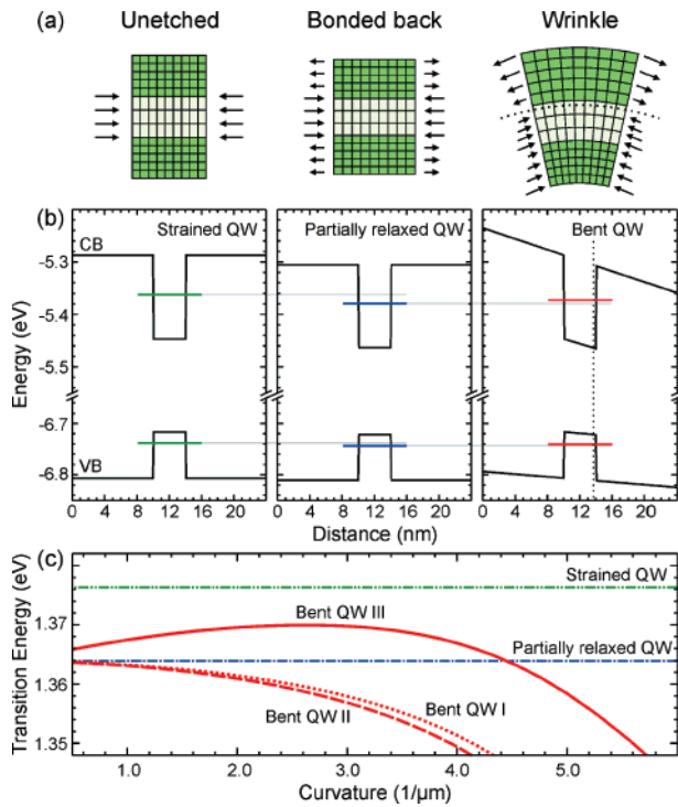
Figure 3. (a) Schematic of the unetched (strained QW), bonded back (partially relaxed QW), and wrinkle (bent QW) structures. Arrows represent the force applied to the layer, and the dotted line in the wrinkle structure indicates the neutral plane. (b) Band diagram corresponding to the structure shown in (a). The lines in the middle of the QW show the quantized energy levels of the electron in conduction band (CB) and heavy hole in the valence band (VB). Light-gray lines are guides to the eyes. (c) Transition energy of the bent QW as a function of the bending curvature. The dashed-dotted-dotted and the dashed-dotted lines represent the transition energy of the strained QW and partially relaxed QW, respectively. Three bent QW models are presented (see text for details).
